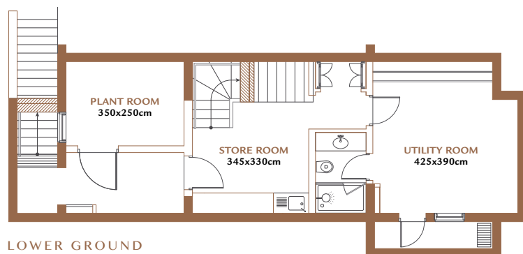
LOWER GROUND
